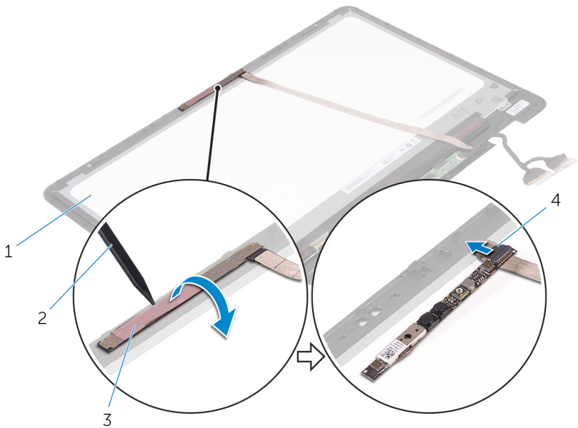
Figure 39. Removing the camera
