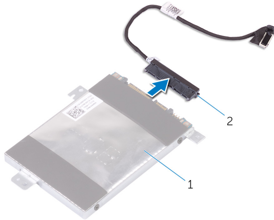
Figure 10. Removing the interposer
