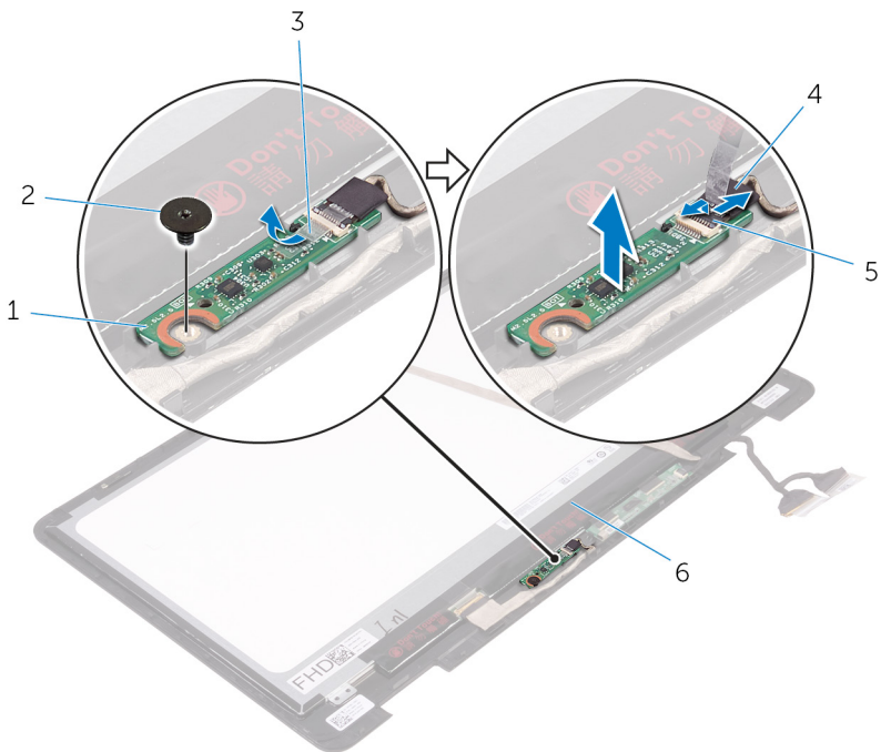
Figure 40. Removing the sensor-board cable
