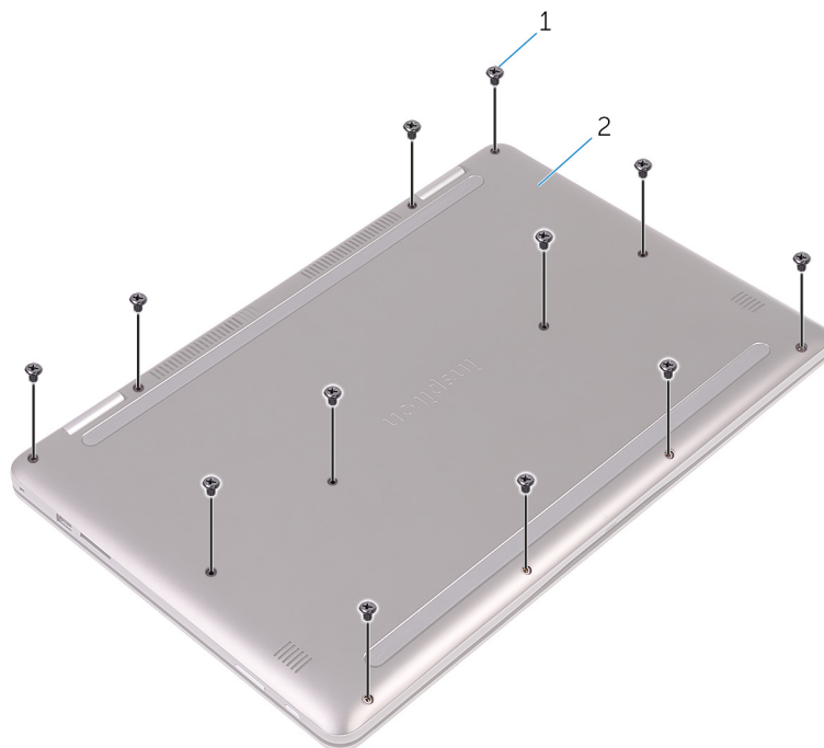
Figure 1. Removing the screws
