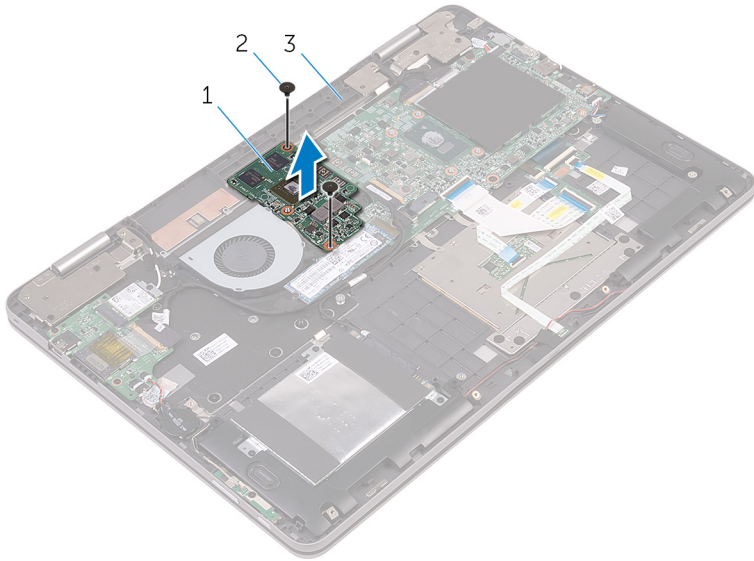
Figure 24. Removing the graphics daughter-board
