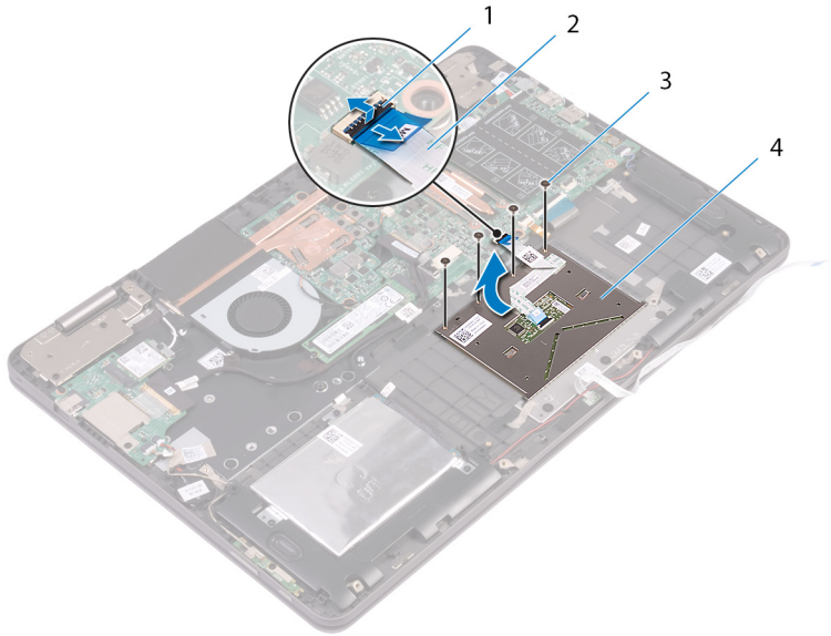
Figure 18. Removing the touchpad
